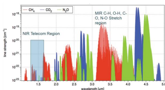
Mid-infrared and near-infrared absorption line intensities
